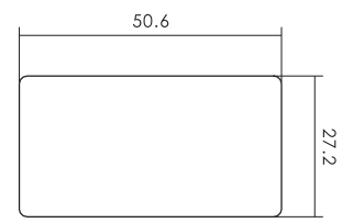
PANEL CUT-OUT
