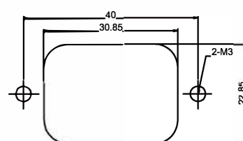
PANEL CUT-OUT
