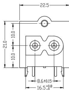
VIEW "B"
