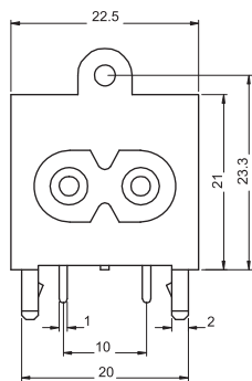
VIEW "A"
